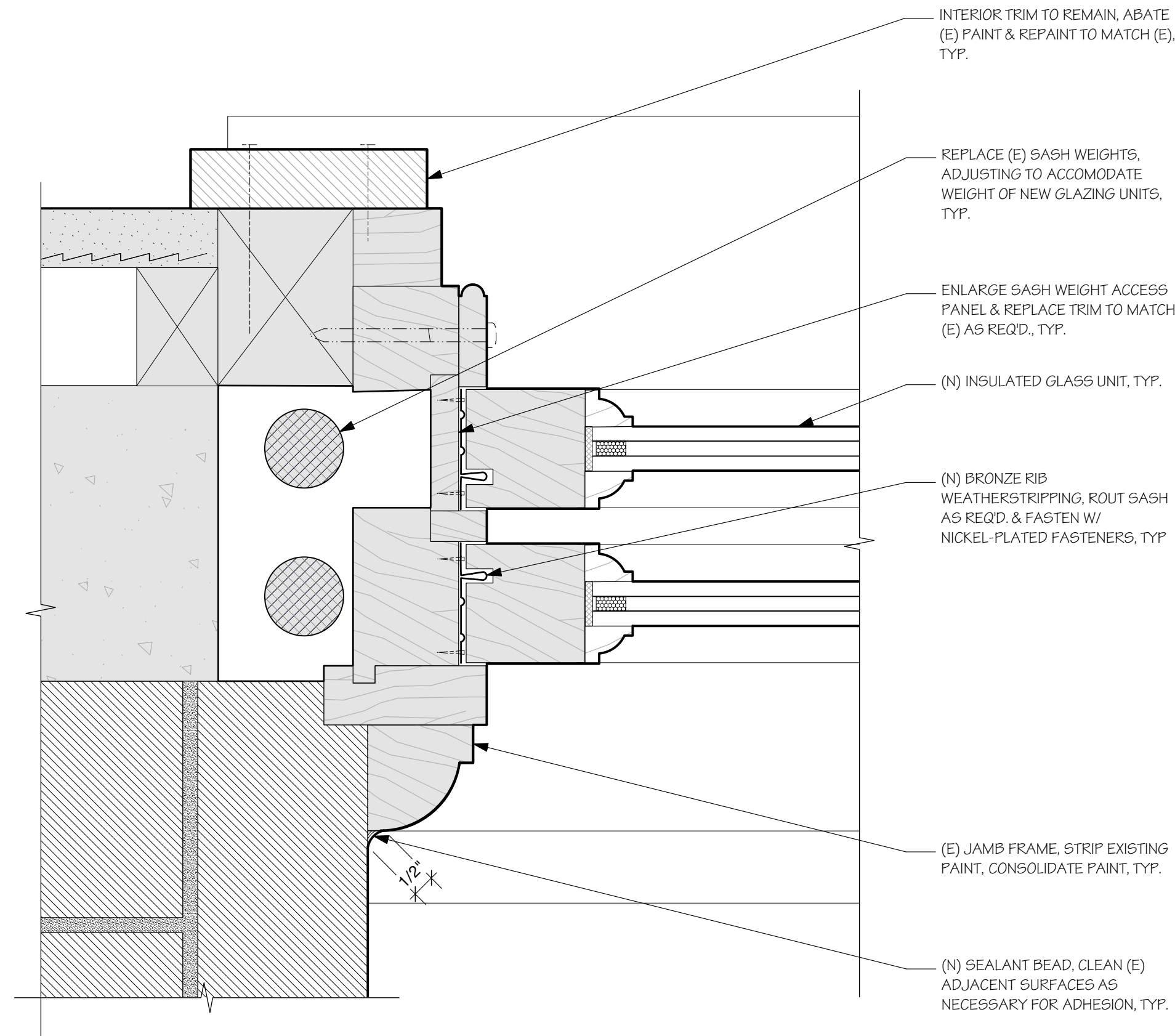
2 (E) WOOD WINDOW JAMB HALF-SIZE
