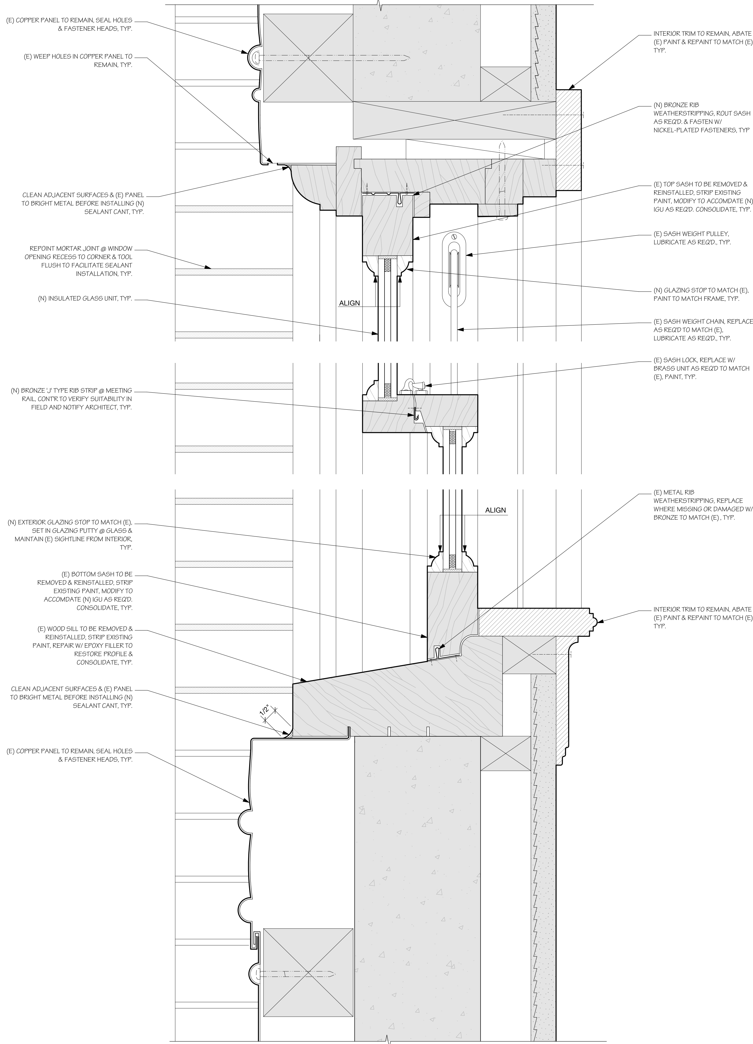
1 (E) WOOD WINDOW SILL & HEAD HALF-SIZE
